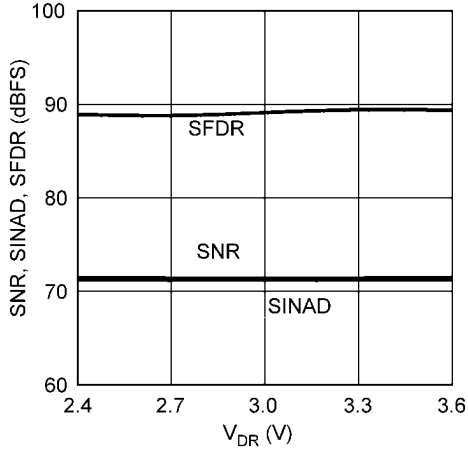
SNR, SINAD, SFDR vs. V_{DR}
