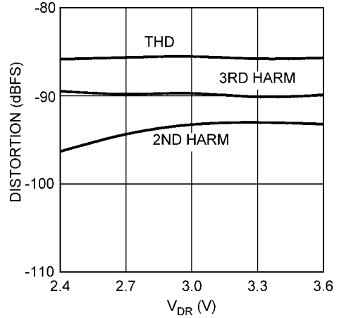
Distortion vs. V_{DR}
